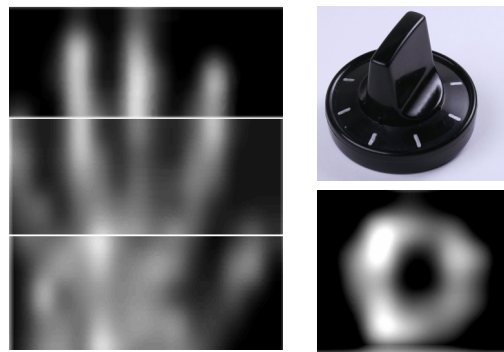
Figure 4: Left, an image of a user’s hand captured through a ThinSight display (based on concatenation of three images captured from the display). A physical dial interface widget (top right) sensed on the surface (bottom right). Note these are the rescaled interpolated images.
