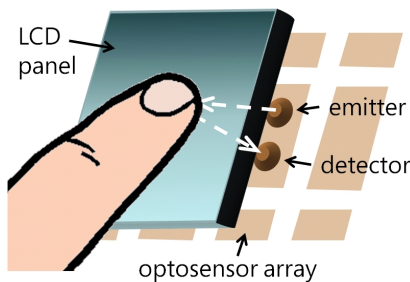
Figure 2: The basic construction of ThinSight. An array of retro-reflective optosensors is placed behind the LCD panel. Each of these contains two elements: an emitter which shines IR light through the panel; and a detector which picks up any light reflected by objects such as fingertips in front of the screen.
