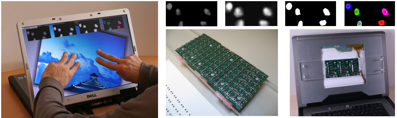
Figure 1: ThinSight enables multi-touch sensing using novel hardware embedded behind an LCD. Left, multi-touch input on a regular laptop LCD. Top row, the sensor data after interpolation, normalization, binarization, and component analysis. Bottom middle, front of three sensor boards tiled. Bottom right, sensors in position behind the display.
