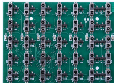
Figure 3: The front side of the sensor PCB showing the 7x5 array of IR optosensors. The transistors that enable each detector are visible to the right of each optosensor. Three such PCBs are used in our ThinSight prototype.
